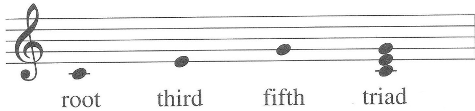
Fig. 1: C triad
